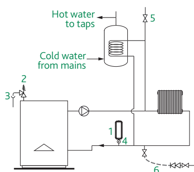
Fig. 3 - Typical System
